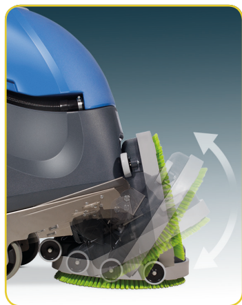
Deck tilt system
